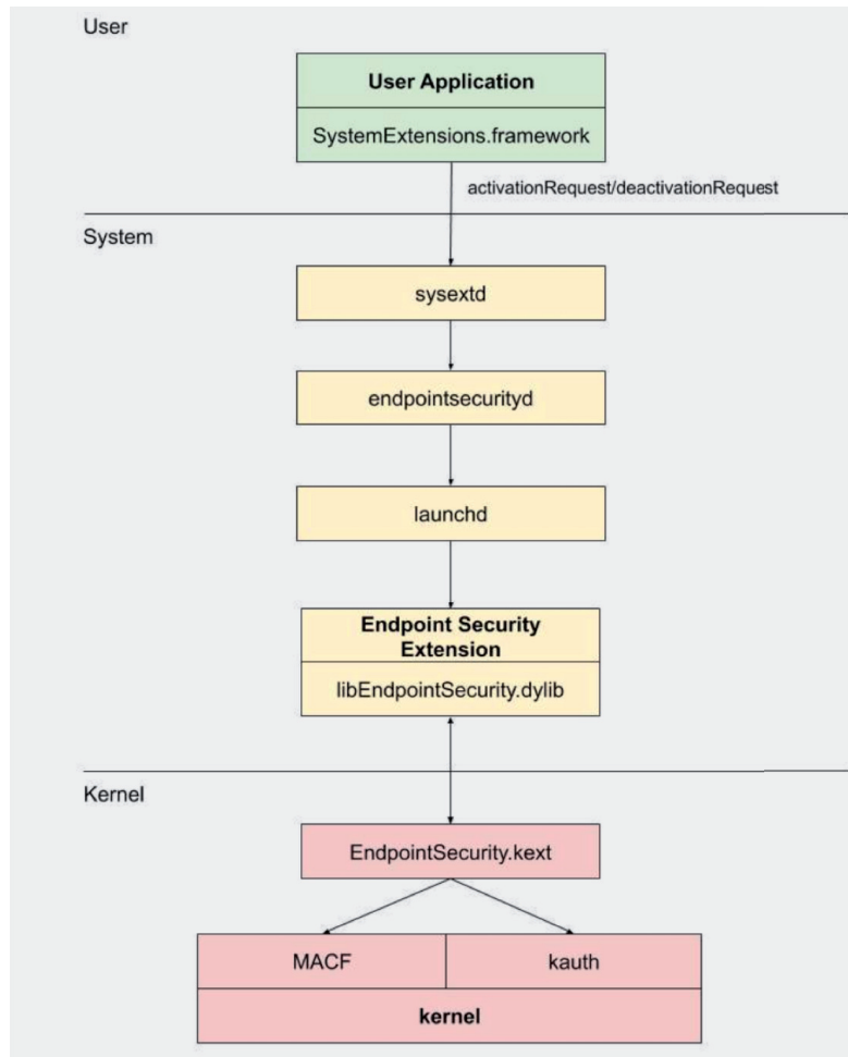
Figure 2: Framework architecture.
